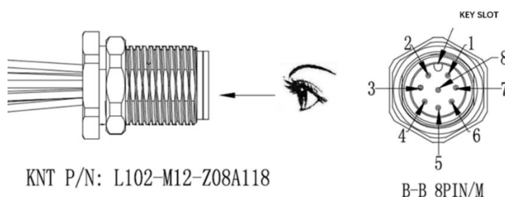
Figure 2.1 Cable Connector on the Lidar Base
