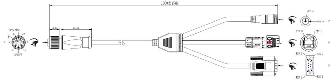
Figure 2.2 Adapter Cable
