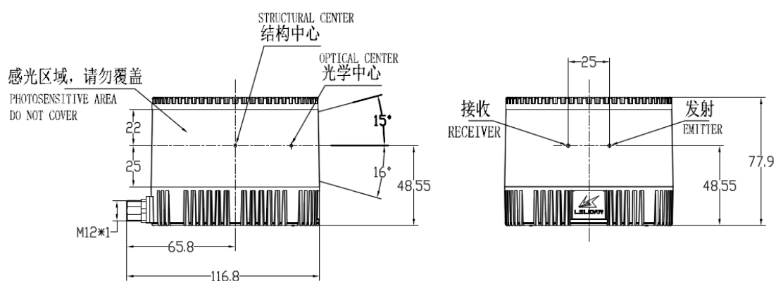
Figure 1.7 C32 Mechanical Drawing (unit: mm) (cable interface at side)
