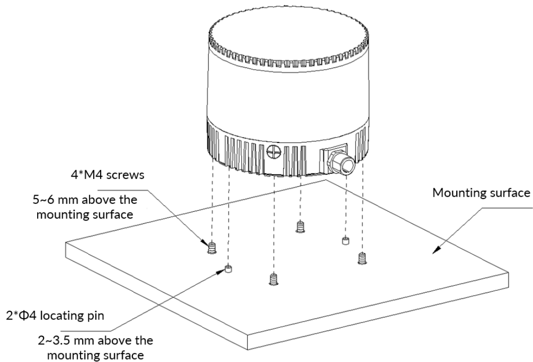
Figure 1.9 LiDAR Mounting Reference Drawing
